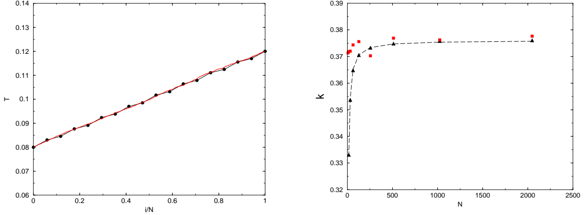
Figure 2: Results of simulations for K = 1 . Left: temperature profile with two heat baths for N = 16 (circles) and N = 2048 (full line). Right: Heat conductivity versus the chain length N obtained through non equilibrium simulations (squares) and GK formula (triangles). The continuous line represents the best fit with a function k_\infty + a/N .
