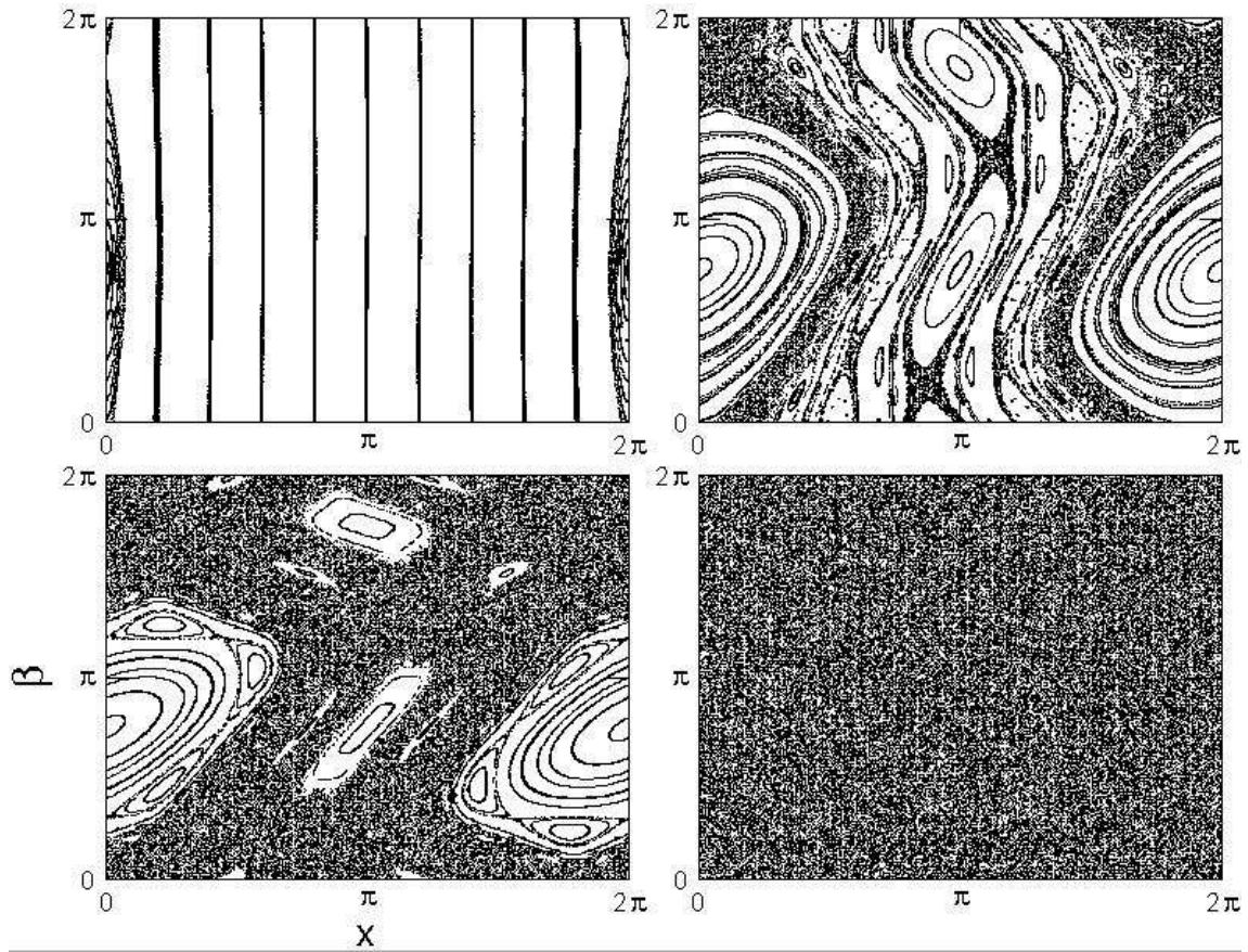
Figure 1: Poincare sections for the map (19). Here K = 1 and v = 0.01 (top left), v = 0.6 (top right), v = 1 . (bottom left), v = 5 . (bottom right)
