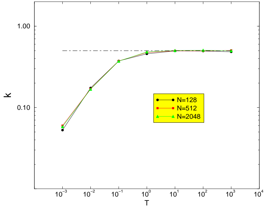
Figure 3: Thermal conductivity k versus the temperature (note the log-log scale). The dashed line corresponds to the value k = 1/2 . Results are plotted for three different N values (see legend). Here only a single trajectory has been used in the application of the Green-Kubo formula. However the good overlap between the three curves indicates reliability of the computation.
