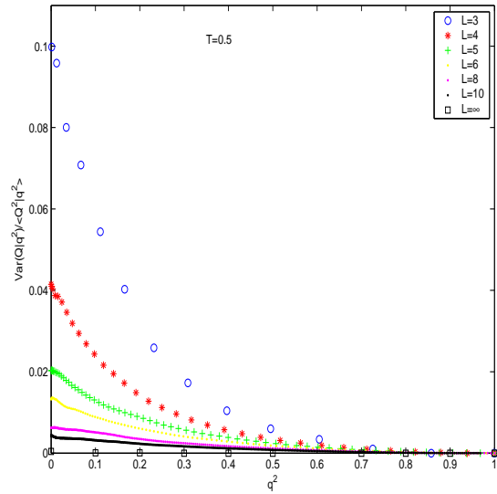
Figure 4: Var(Q|q^2)_{L,T} / \langle Q^2|q^2 \rangle as a function of q^2 for the temperature T = 0.5 and for different sizes L together with the infinite volume limit.
