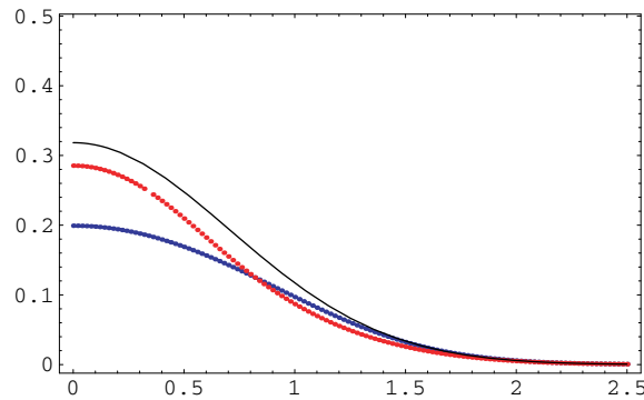
Figure 4. A_{SK}(h) (bottom), A_{ROM}(h) (middle) and \frac{1}{\pi} e^{-h^2} (top). (This figure is in colour only in the electronic version)
