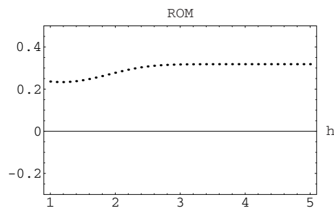
Figure 5. Plot of e^{h^2} A_{ROM}(h) for values of the magnetic field h between 1 and 5.
